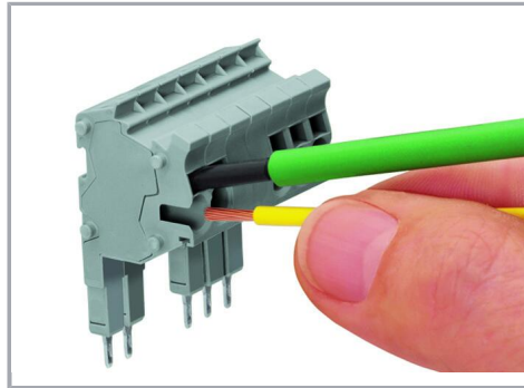
Conductor termination via:
