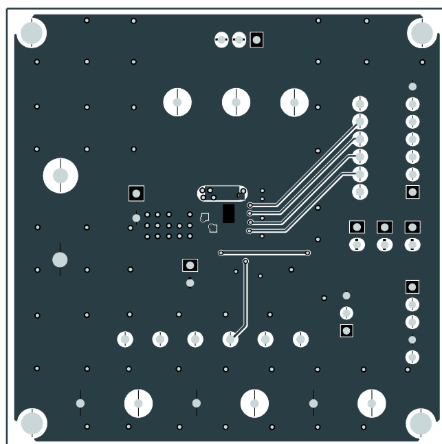
Figure 4: Bottom Layer
