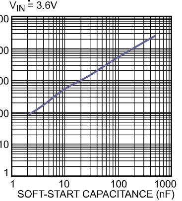
Soft-Start Time vs. Soft-Start Capacitance
