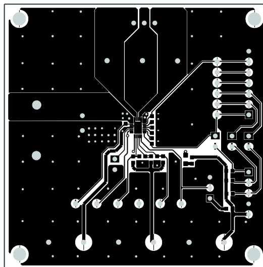
Figure 3: Top Layer
