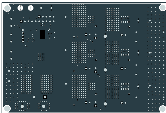
Figure 5: Inner Layer 2
