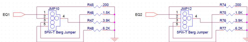
Figure 3. Early Board JMP10 and JMP12 Schematic
