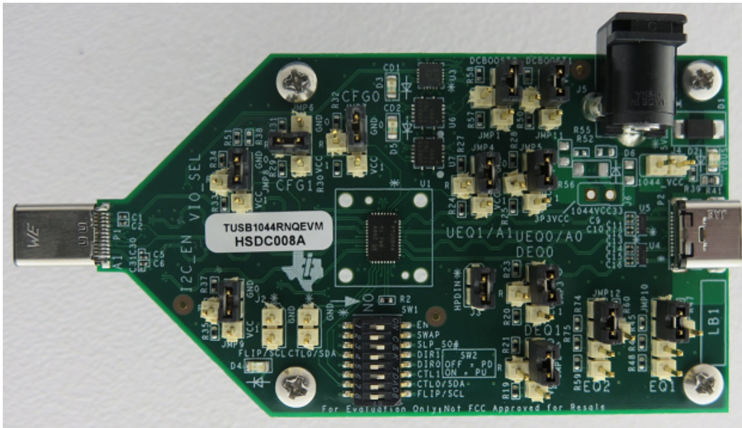
Figure 1. TUSB1044 EVM
