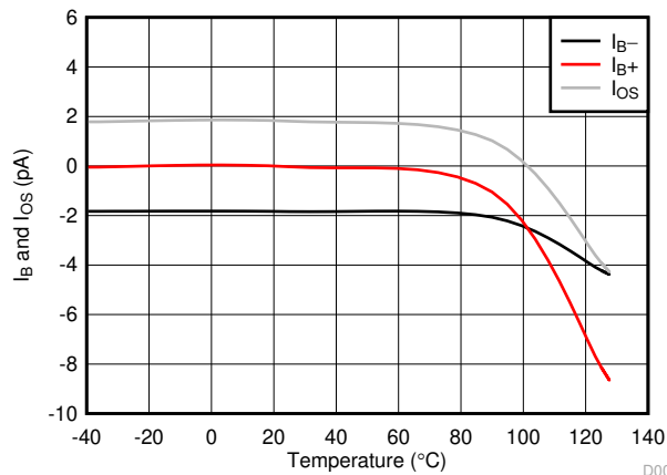
Figure 6-1. I_B and I_{OS} vs Temperature
