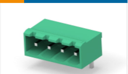
TE Part #2350513-4 4POS TB HDR 90 DEG, PITCH 5.0 & TL 4.5mm
