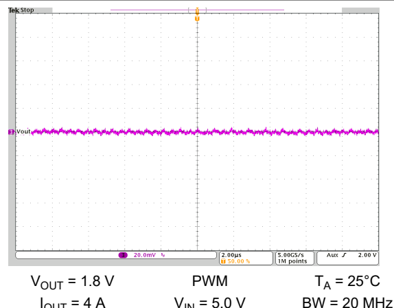
Figure 10-45. Output Voltage Ripple
