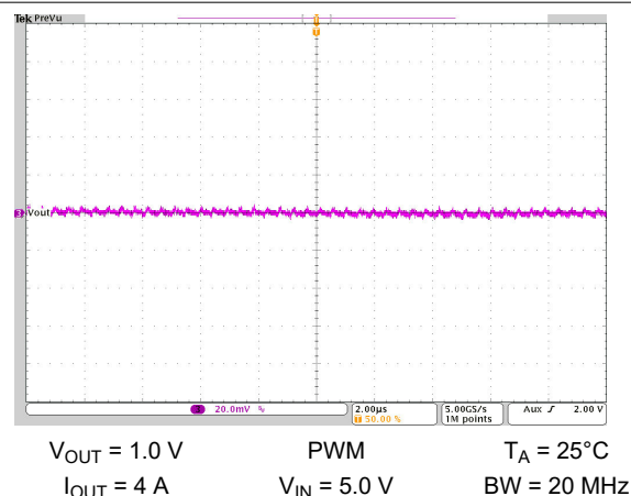
Figure 10-49. Output Voltage Ripple
