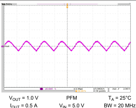
Figure 10-48. Output Voltage Ripple
