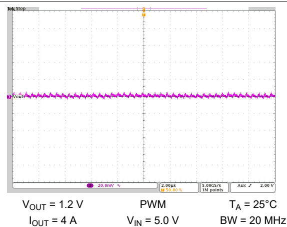
Figure 10-47. Output Voltage Ripple
