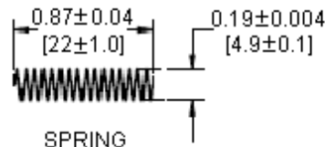
SPRING
