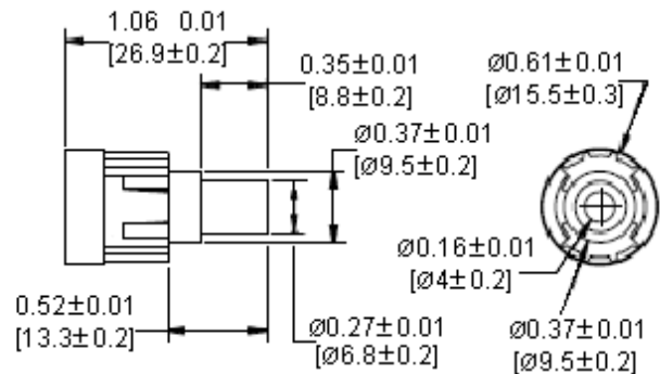
TOP PART
