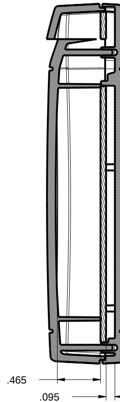
SECTION S-S
