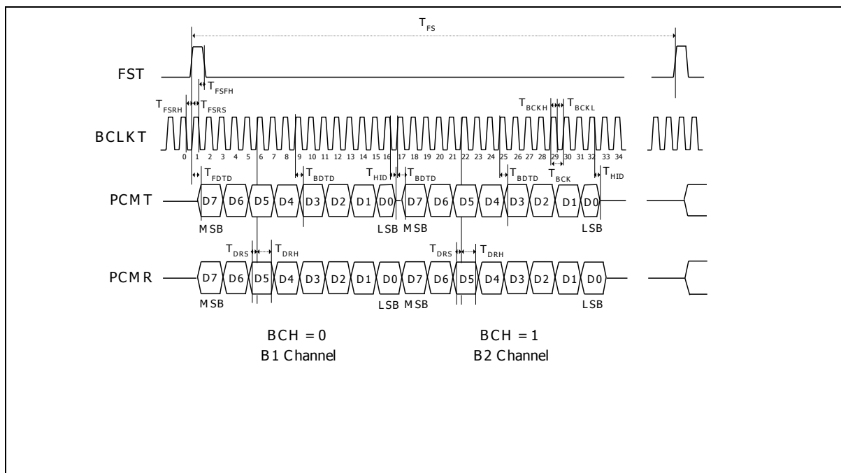
Figure 8.4 GCI PCM Timing
