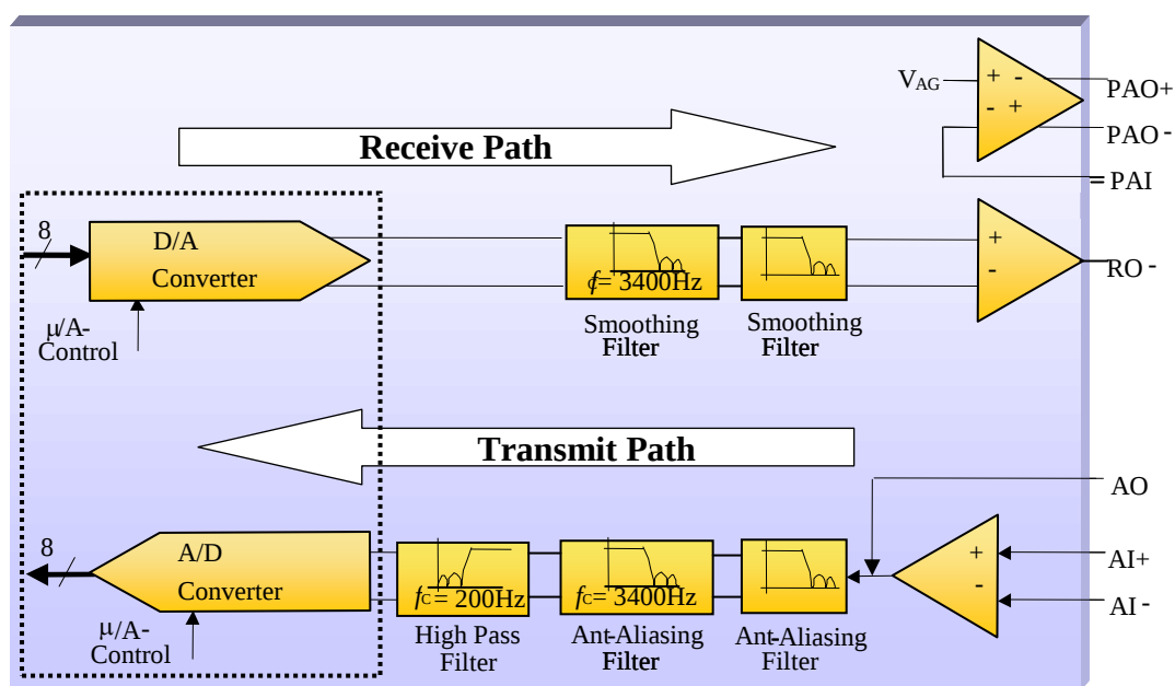
Figure 7.1 The W6811 Signal Path
