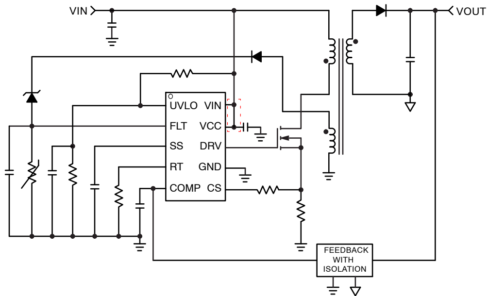
Figure 2. Typical Application Circuit for Vin = 9 – 18 V
