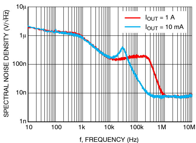
Figure 11. Output Voltage Spectral Noise Density vs. Frequency – V_{OUT(NOM)} = 1.8\text{ V}
