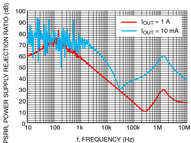
Figure 9. V_{IN} PSRR vs. Frequency V_{OUT(NOM)} = 1.8\text{ V}
