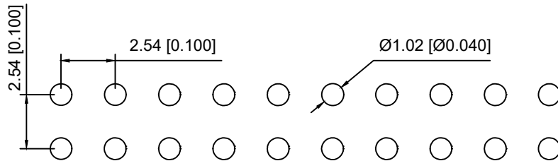
PCB LAYOUT
