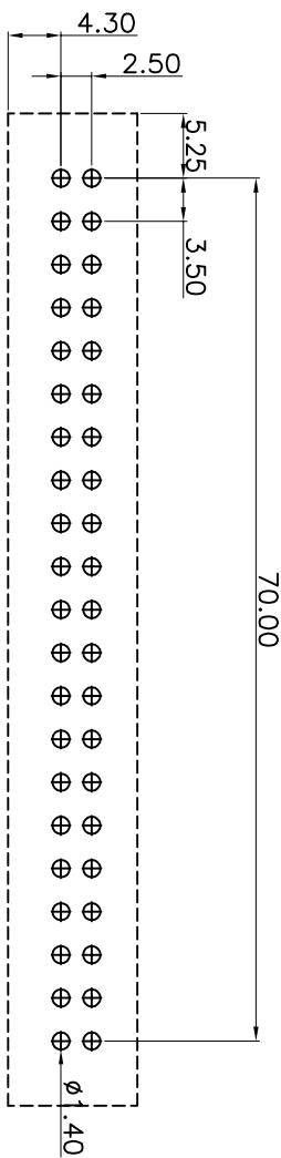
PCB LAYOUT
