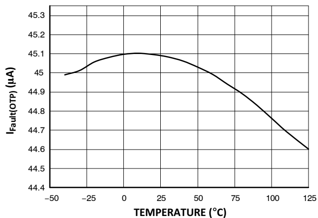
Figure 26. I Fault(OTP) vs. Junction Temperature
