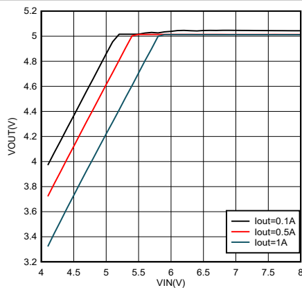
f_{SW} = 2.1\text{ MHz} V_{OUT} = 5\text{ V} LMR54410
