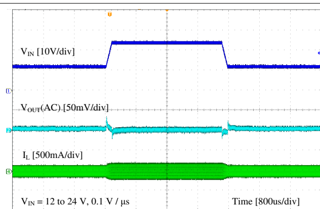
Figure 9-8. Line Transient
