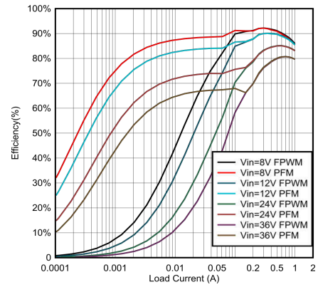
Figure 7-2. 3.3-V Efficiency Versus Load Current - LMR54410
