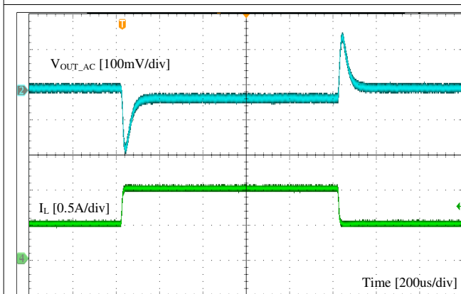
Figure 9-7. Load Transient
