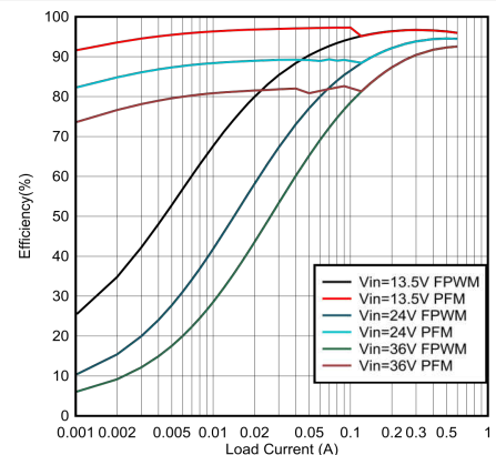
Figure 7-4. 5-V Efficiency Versus Load Current
