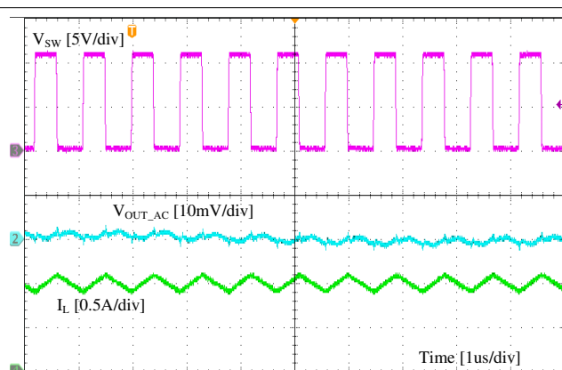
Figure 9-4. Ripple at Full Load
