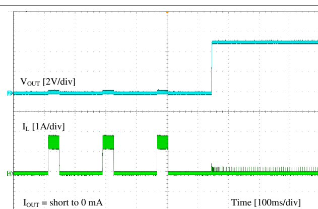
Figure 9-10. Short Recovery
