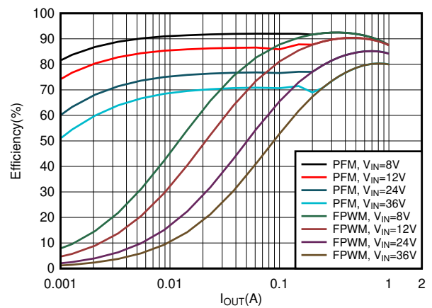
Figure 7-4. 5-V Efficiency Versus Load Current
