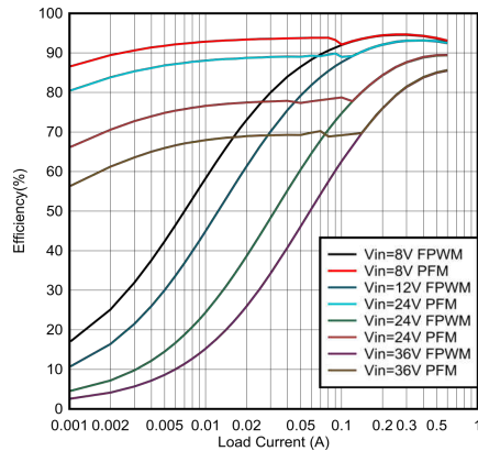
Figure 7-1. 3.3-V Efficiency Versus Load Current - LMR54406
