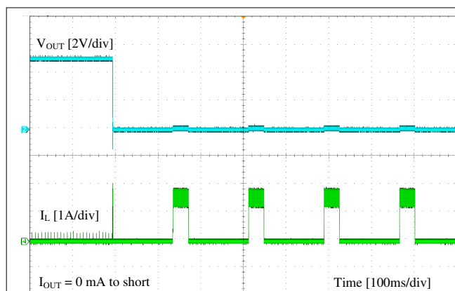
Figure 9-9. Short Protection
