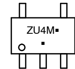
SC-88A CASE 419A-02
