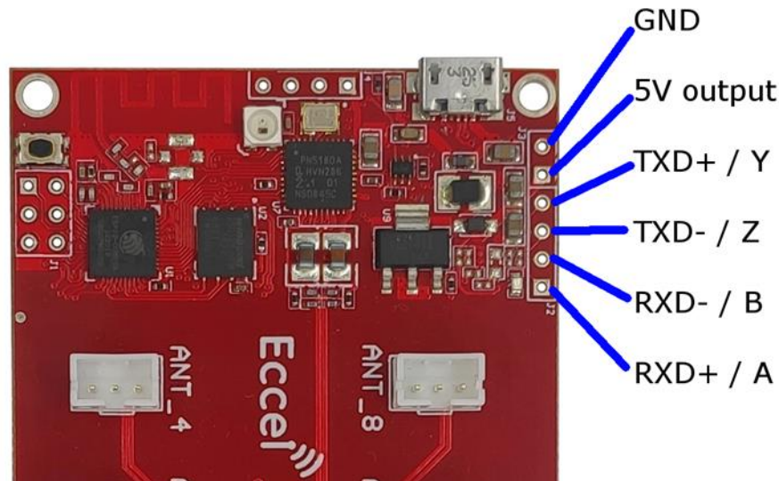
Figure 9-1 RS-485 pinout
