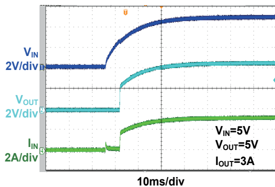
V_{IN} On (5V IN , I O =3A)
