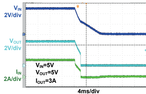
V_{IN} Off (5V IN , I O =3A)
