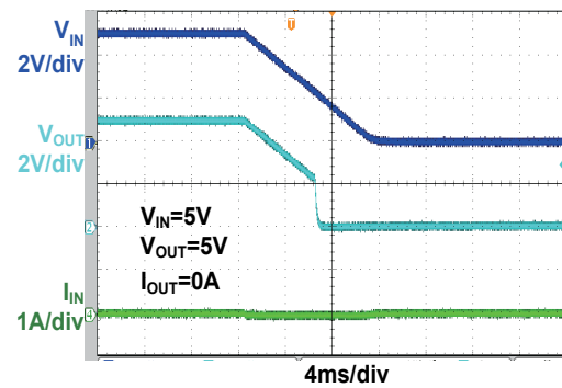
V_{IN} Off (5V IN , I O =0A)
