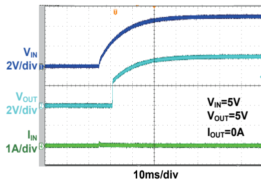
V_{IN} On (5V IN , I O =0A)
