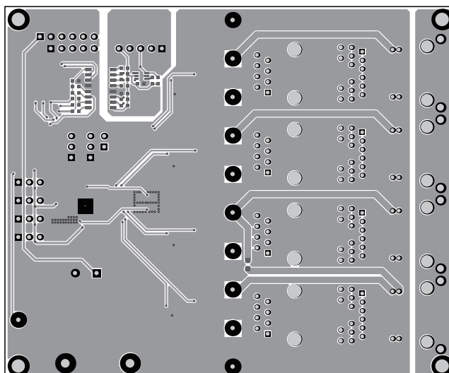
Figure 4: Bottom Layer
