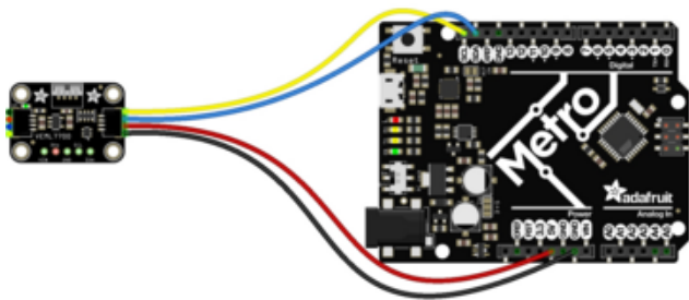
fritzing
