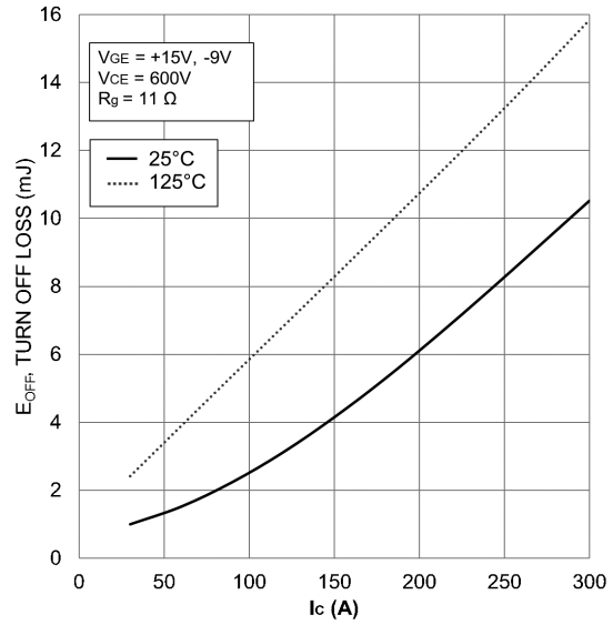
Figure 22. Typical Turn Off Loss vs. I_C
