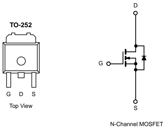
N-Channel MOSFET
