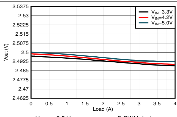
Figure 9-18. Load Regulation
