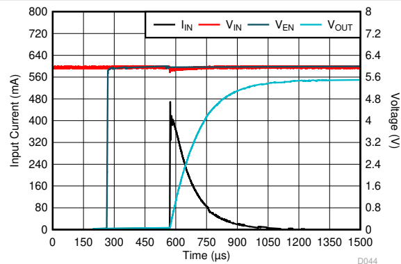
Figure 6-85. Inrush Current
