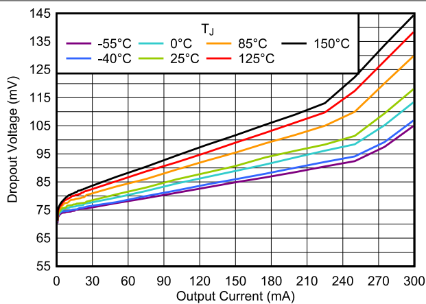
Figure 6-25. Dropout Voltage vs I_{OUT}
