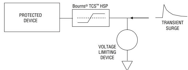
Coordination of Bourns® TCS™ High-Speed Protector with Overvoltage Limiting Device
