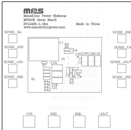
Figure 1: Top Silk
