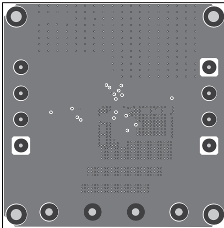
Figure 3: Mid-Layer 1
