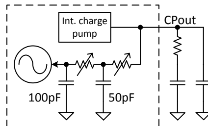
Figure 7-2. Integrated Loop Filter
