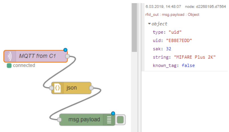
Figure 4-5 Node-Red – the MQTT client + JSON frame example
