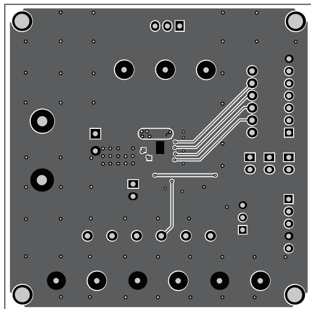
Figure 5: Bottom Layer
