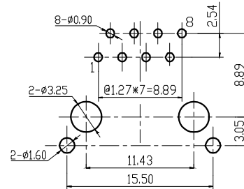
PC Board Layout thickness=1.6mm
