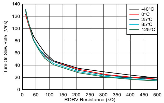
Figure 7-4. Turn-On Slew Rate vs Drive Strength Resistance
