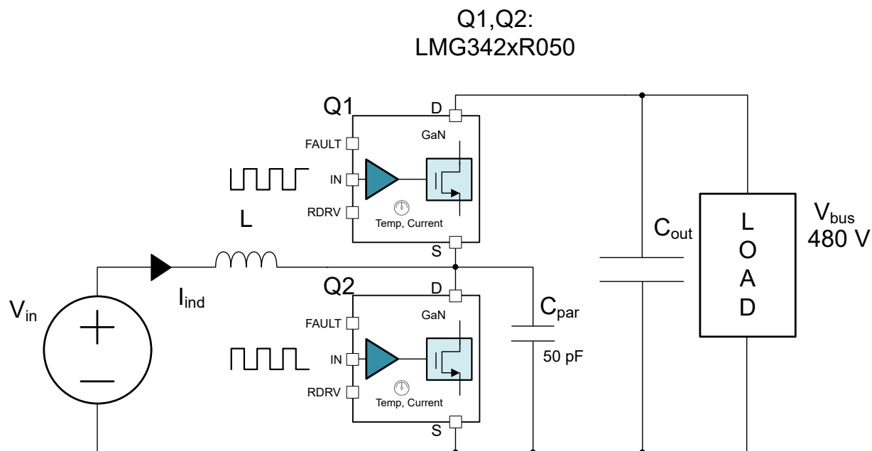
Figure 9-9. Circuit Used for SOA Curve
