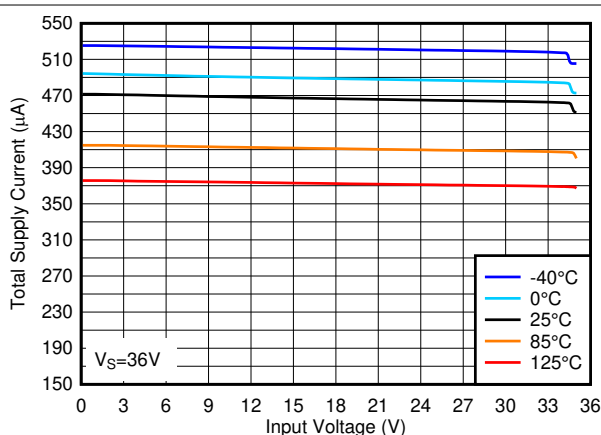
Figure 3-12. Total Supply Current vs. Input Voltage at 36V
