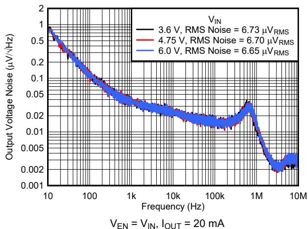
Figure 6-38. Noise vs Frequency and V_{IN}
