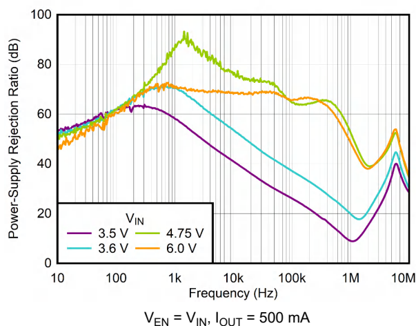
Figure 6-35. PSRR vs Frequency and V_{IN}
