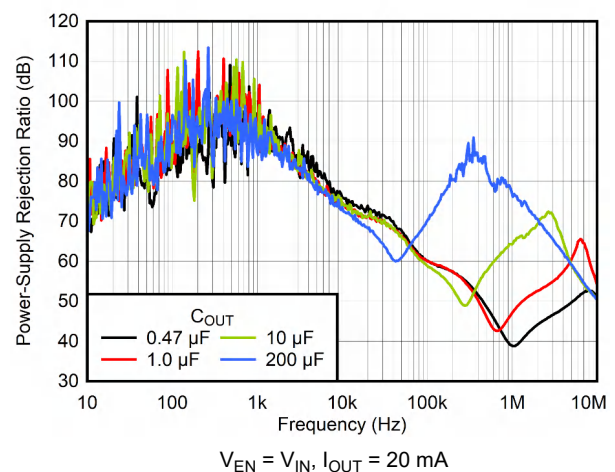
Figure 6-36. PSRR vs Frequency and C_{OUT}
