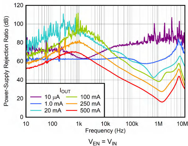
Figure 6-33. PSRR vs Frequency and I_{OUT}
