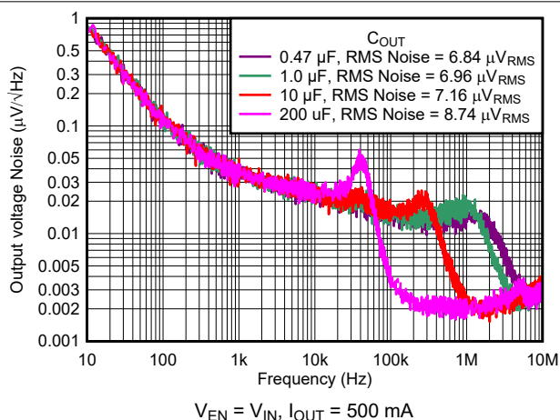
Figure 6-42. Noise vs Frequency and C_{OUT}
