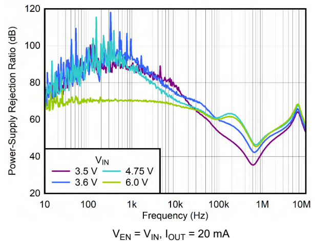
Figure 6-34. PSRR vs Frequency and V_{IN}
