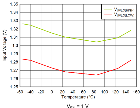
Figure 6-19. V_{IN} UVLO Threshold vs Temperature
