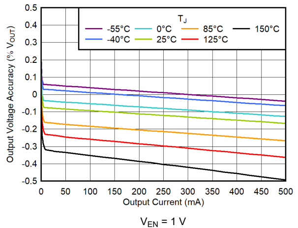
Figure 6-2. Output Voltage Accuracy vs I_{OUT}
