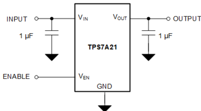
Simplified Schematic
