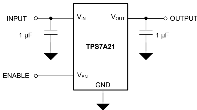
Figure 8-4. TPS7A21 Typical Application
