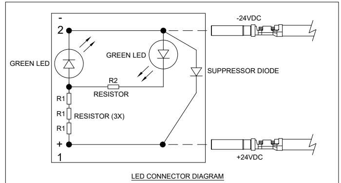
LED CONNECTOR DIAGRAM
