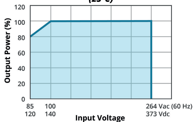
INPUT VOLTAGE DERATING CURVE (25°C)
