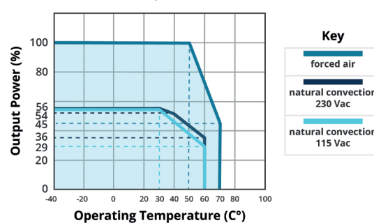
TEMPERATURE DERATING CURVE (full load 550W with 25 CFM) VMS-550C-24-CFS, VMS-550C-27-CFS VMS-550C-36-CFS, VMS-550C-48-CFS
