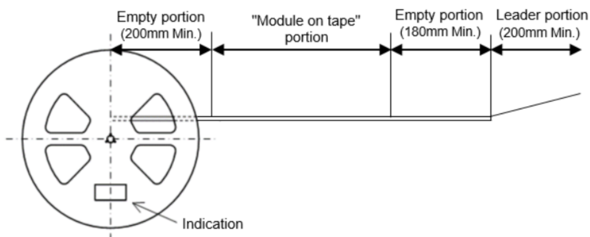
Figure 45. Taping Specification
