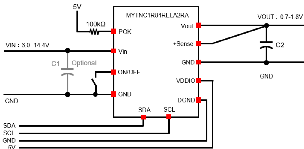
Figure 39. Application Schematic
