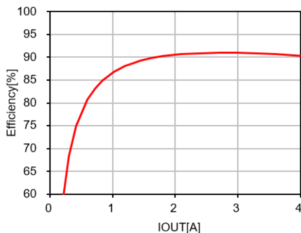
Figure 1. Efficiency Plot
