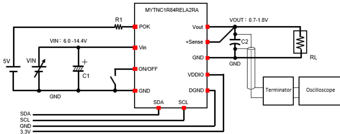
Figure 35. Test Circuit
