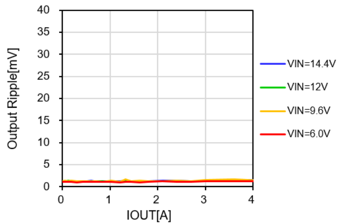
Figure 32. Output Ripple and Noise
