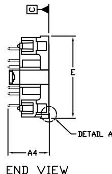
END VIEW
