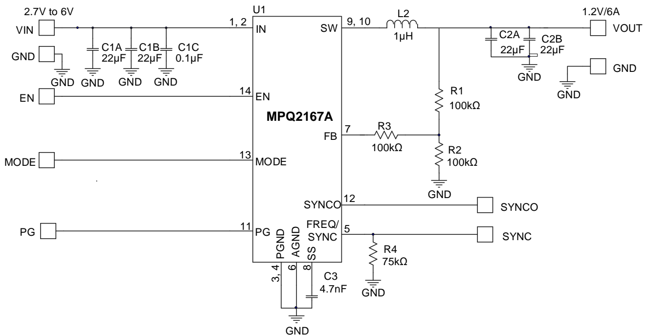
Figure 6: V OUT = 1.2V, I OUT = 6A Application Circuit
