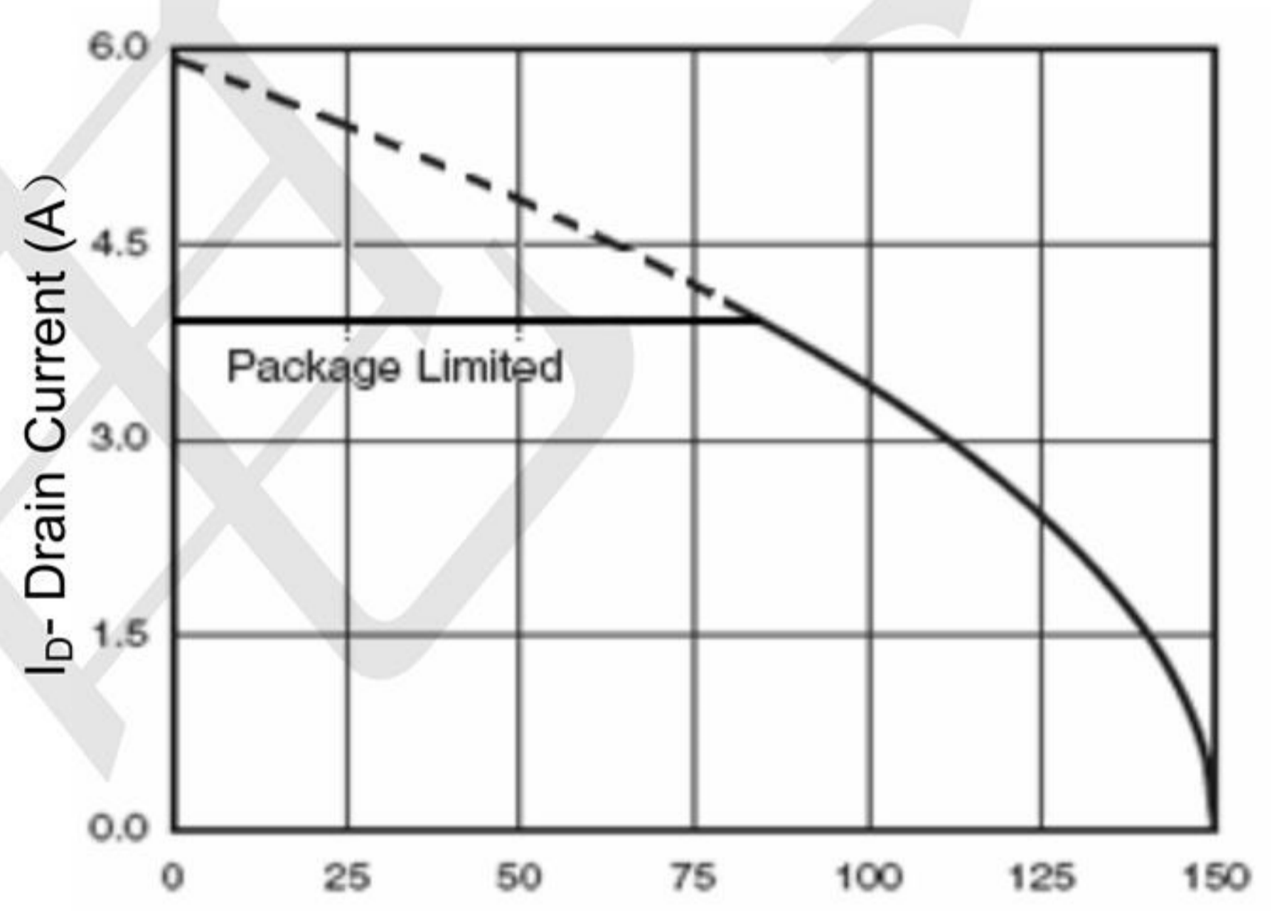
T J -Junction Temperature(°C) Figure 4 Drain Current
