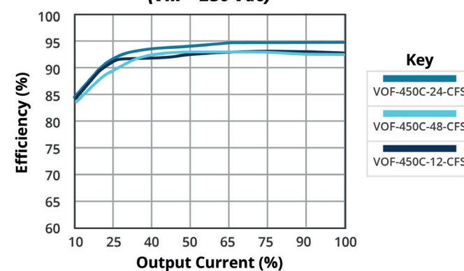
EFFICIENCY VS OUTPUT LOAD ( V_{in} = 230 \text{ Vac} )
