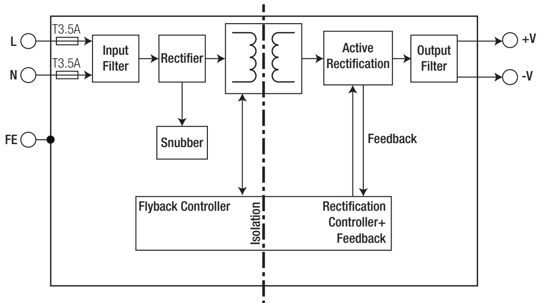
Blockdiagram ("OF/2x4")
