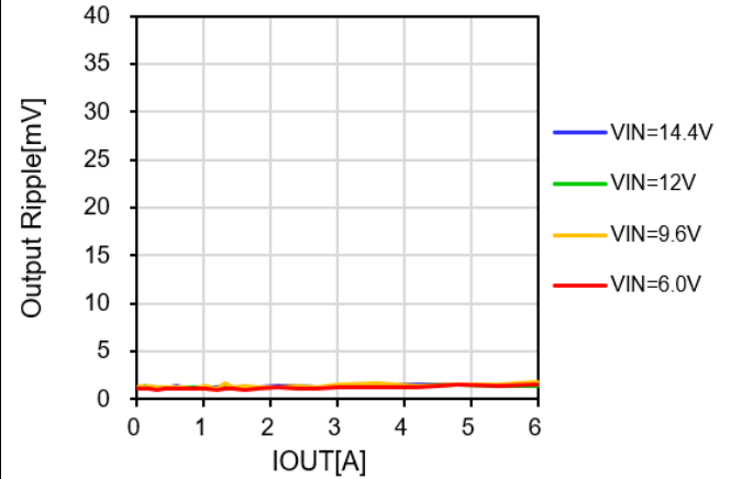
Figure 32. Output Ripple and Noise
