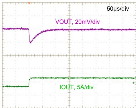
Figure 33. Step Load Transient Response
