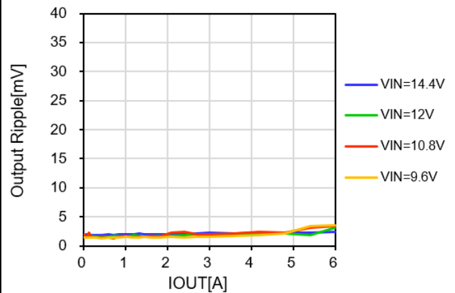
Figure 20. Output Ripple and Noise
