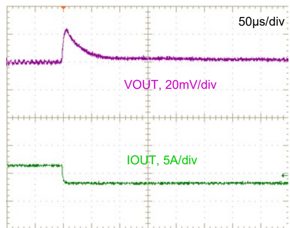
Figure 22. Step Load Transient Response
