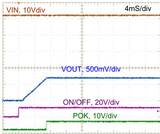
Figure 31. On/Off Enable wave form
