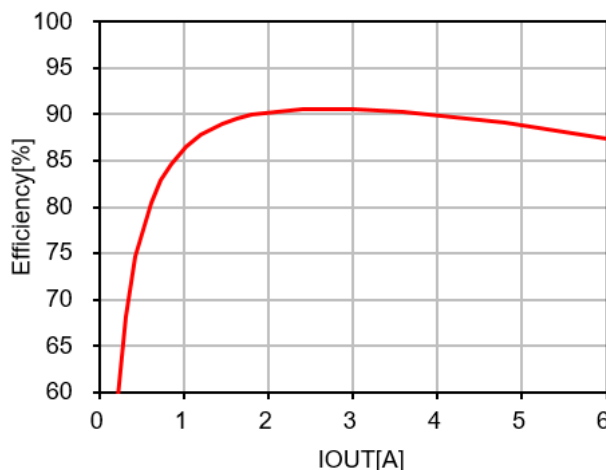
Figure 1. Efficiency Plot
