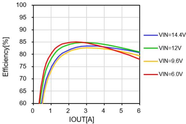
Figure 29. Efficiency vs. Load Current and Line Voltage
