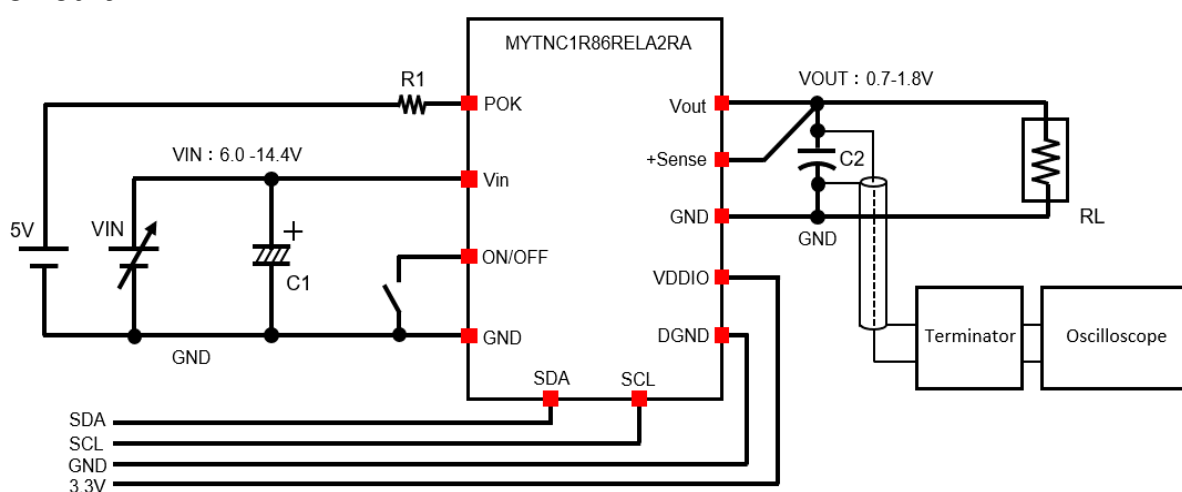
Figure 35. Test Circuit
