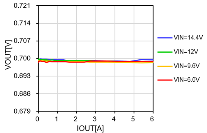
Figure 30. VOUT vs. Load Current and Line Voltage
