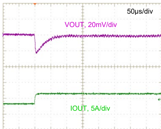
Figure 21. Step Load Transient Response
