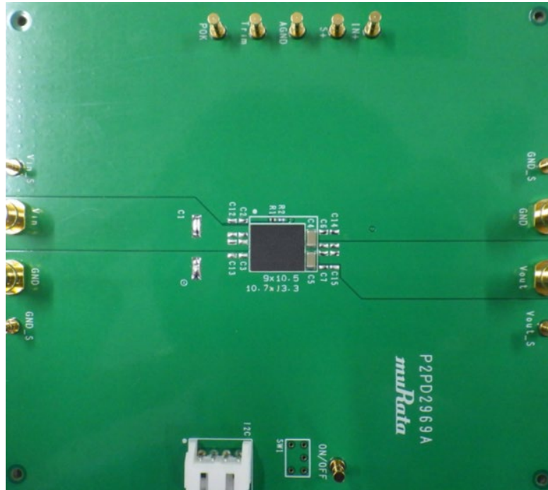
Figure 40. Applicatuin Board Example (Based on JEDEC standard)
