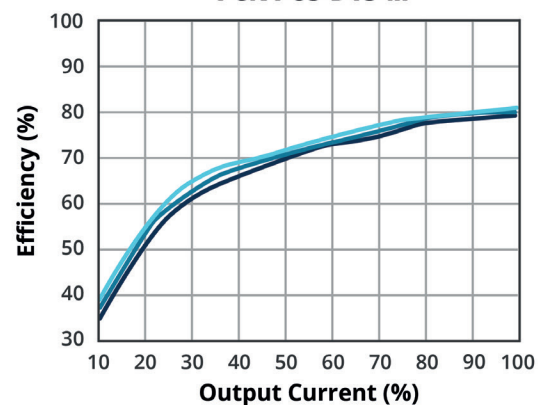
EFFICIENCY VS OUTPUT LOAD PCN1-S5-D15-M
