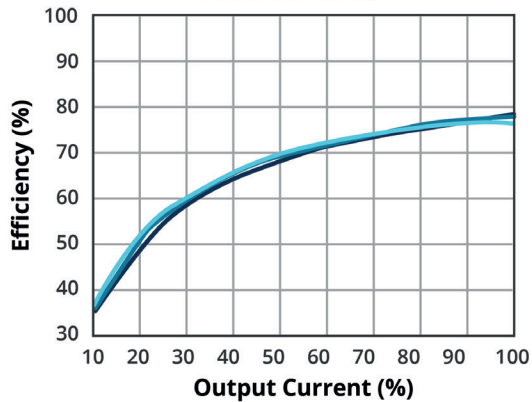
EFFICIENCY VS OUTPUT LOAD PCN1-S5-S5-M
