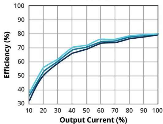
EFFICIENCY VS OUTPUT LOAD PCN1-S5-S15-M
