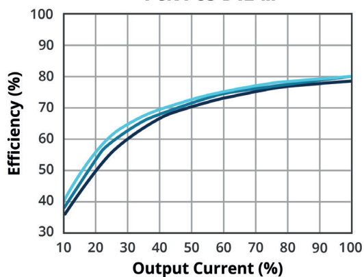
EFFICIENCY VS OUTPUT LOAD PCN1-S5-D12-M
