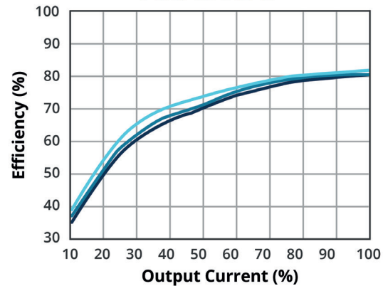
EFFICIENCY VS OUTPUT LOAD PCN1-S5-S12-M
