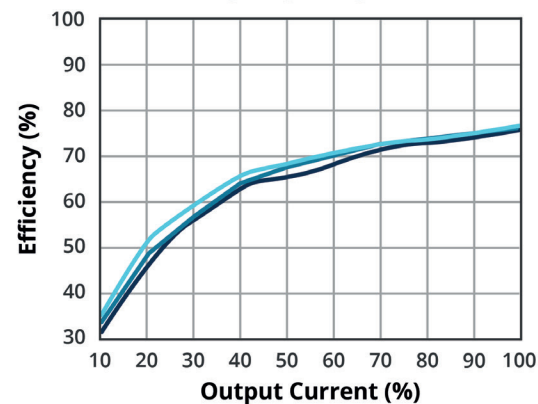
EFFICIENCY VS OUTPUT LOAD PCN1-S12-D5-M
