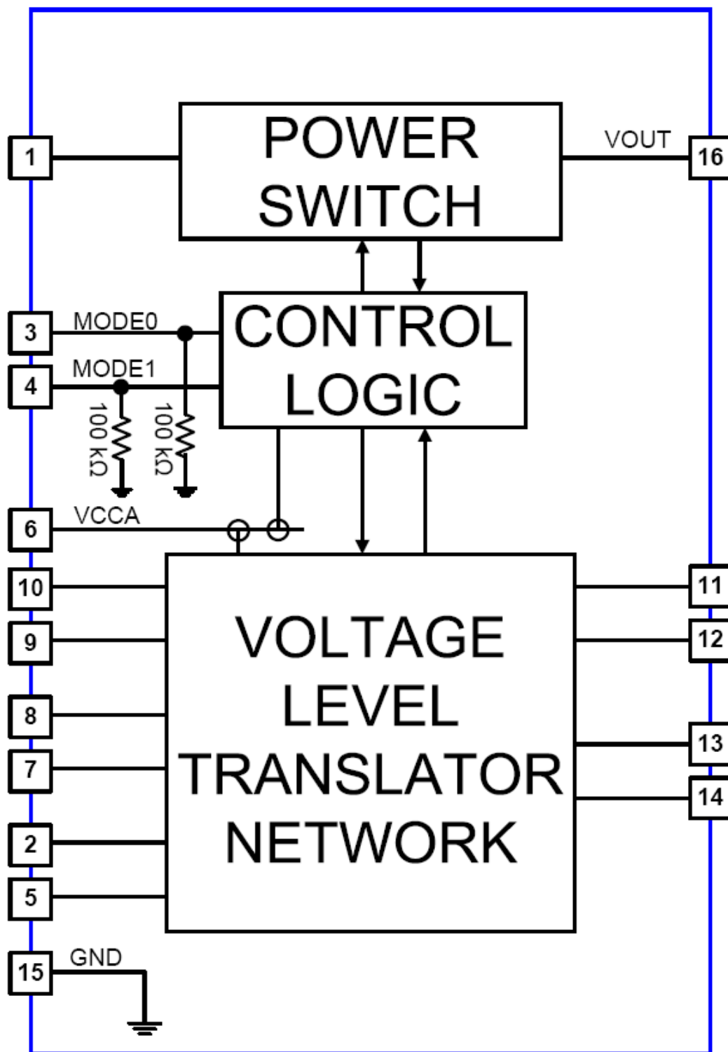
Figure 1. Function Diagram
