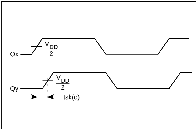
Figure 7. Output Skew
