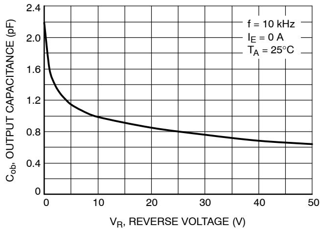
Figure 106. Output Capacitance
